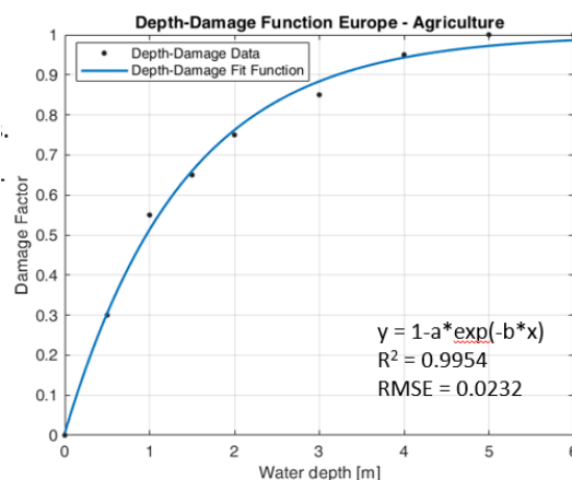
Figure 5-1 – JRC depth-damage curve fitting for the agricultural class for Europe.
